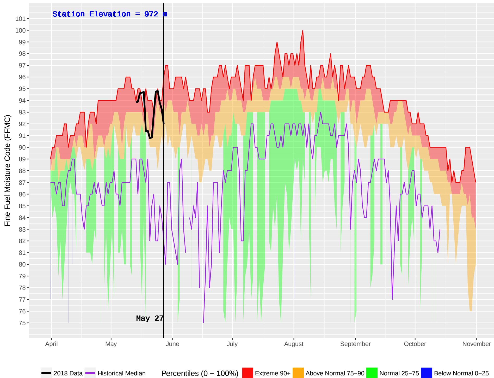
SPARKS LAKE (305) : Historical (1991–2016) and Current (2018) Noon Fine Fuel Moisture Code (FFMC)
