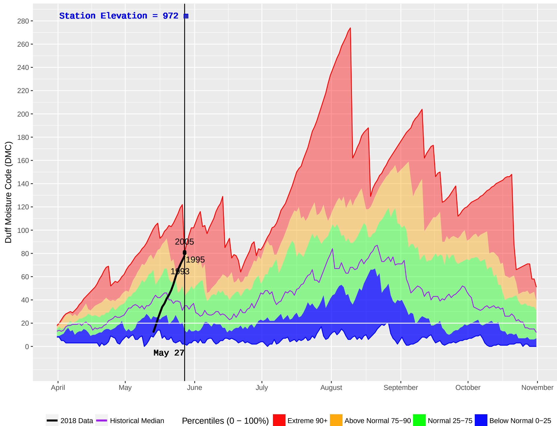
SPARKS LAKE (305) : Historical (1991–2016) and Current (2018) Noon Duff Moisture Code (DMC)
